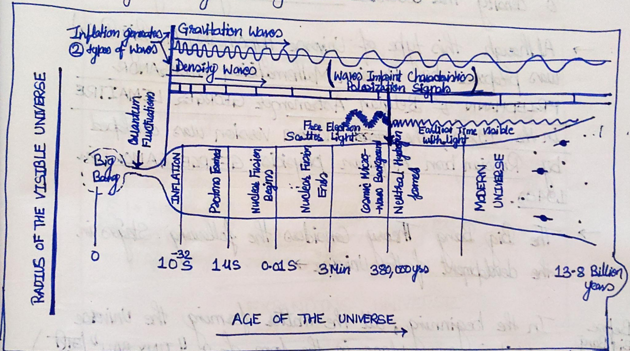
Figure: History of the Universe - gravitational waves arise from Cosmic Inflation, a faster than light expansion just after the Big Bang.
